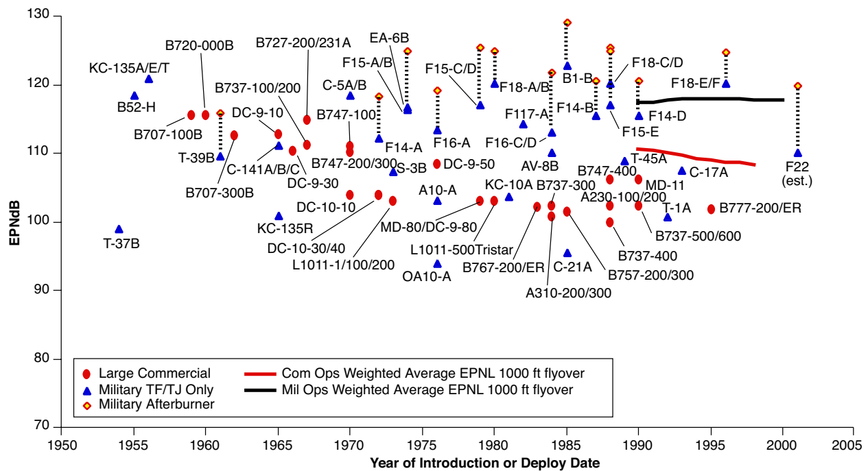
Figure 7. Effective perceived noise level for military and commercial aircraft, 1000 ft (~305 m) flyover operation. 29,34-39 Operations-weighted fleet averages are shown.
